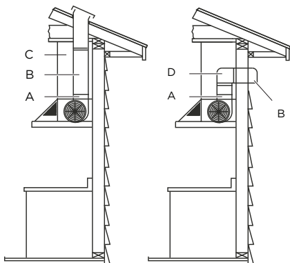
Vertical Discharge
