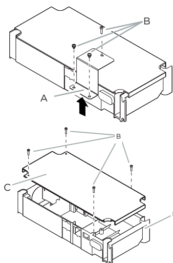
A. Bracket B. Terminal box screws C. Terminal box cover D. Terminal box
