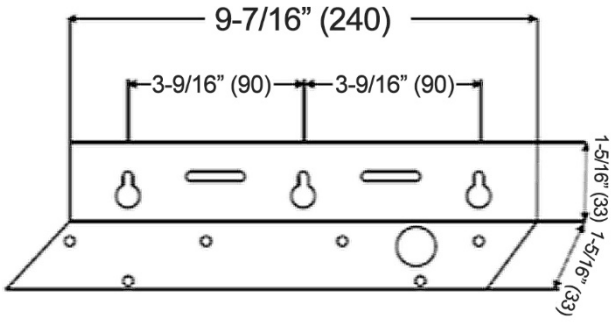
***Hood-Mounting Bracket
